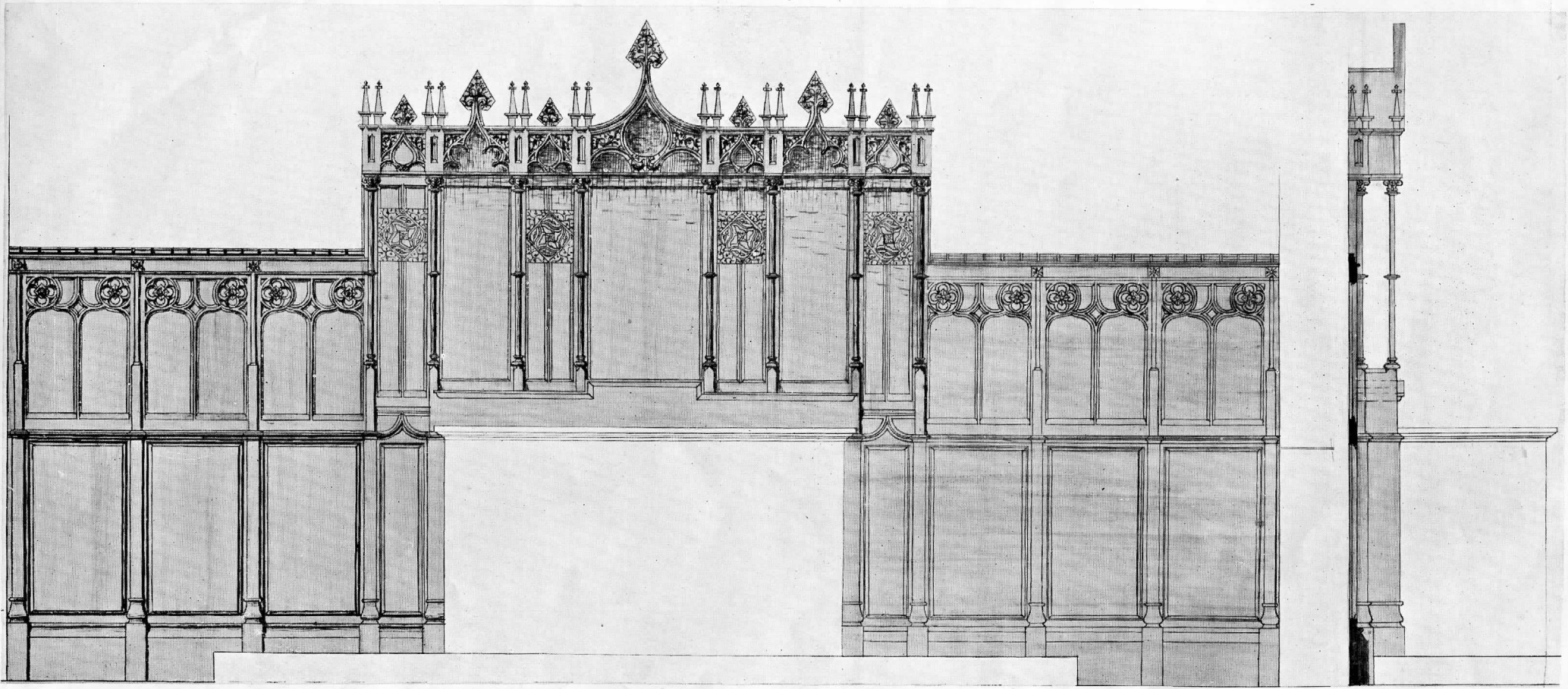
FRONT ELEVATION OF REREDOS
